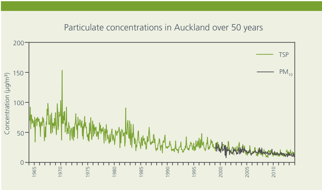
Figure 3.9 Monthly average concentrations of TSP (total suspended particulates) and PM 10 in Auckland over a 50 year period.
