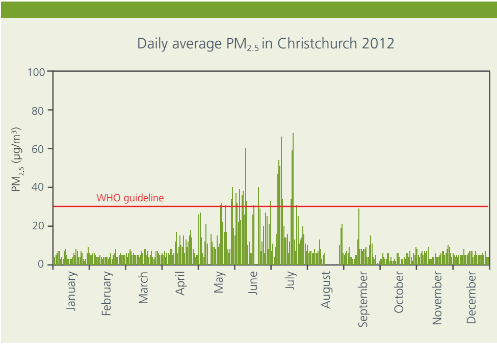
Figure 3.6 Daily concentrations of PM 2.5 measured at the St Albans site in Christchurch in 2012.
