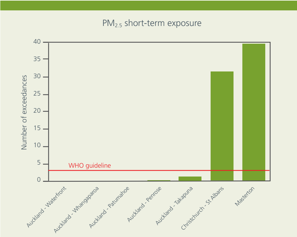
Figure 3.3 Number of days per year on which the concentration of PM 2.5 exceeded 25 µg/m 3 – averaged for the three years 2010–2012 at sites where PM 2.5 has been regularly monitored. Sites above the red line did not ‘pass’ the WHO short-term guideline for PM 2.5 .
