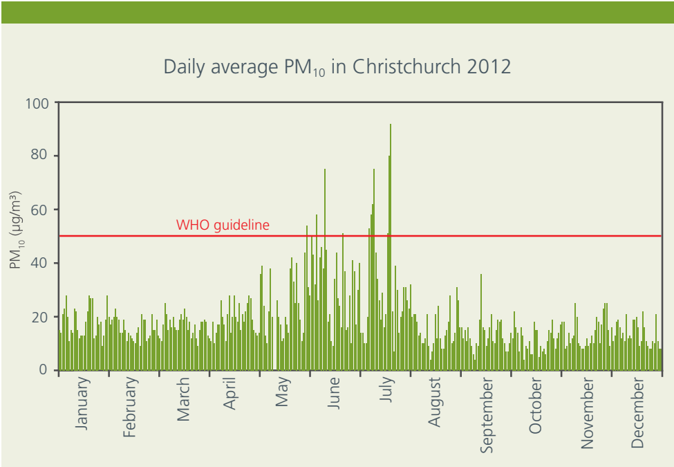
Figure 3.5 Daily concentrations of PM 10 measured at the St Albans site in Christchurch in 2012.
