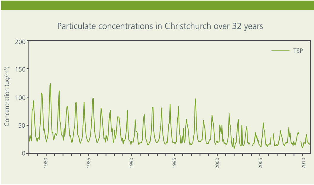
Figure 3.10 Monthly average concentrations of TSP (total suspended particulates) in Christchurch over a 32 year period.
