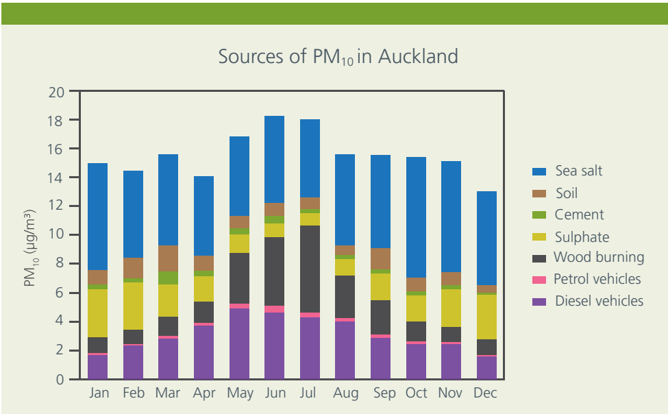
Figure 4.1 Sources of PM 10 at the Takapuna monitoring site in Auckland.
