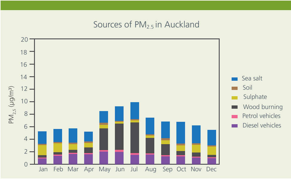
Figure 4.2 Sources of PM 2.5 at the Takapuna monitoring site in Auckland.
