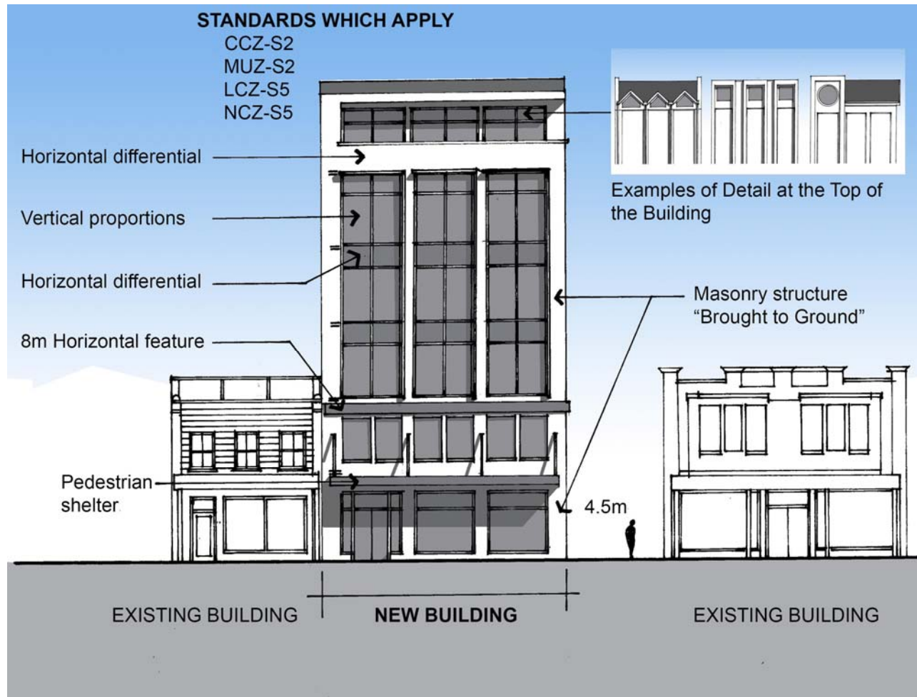
APP20 – Figure 2: Maximum height buildings that face a public road or square
