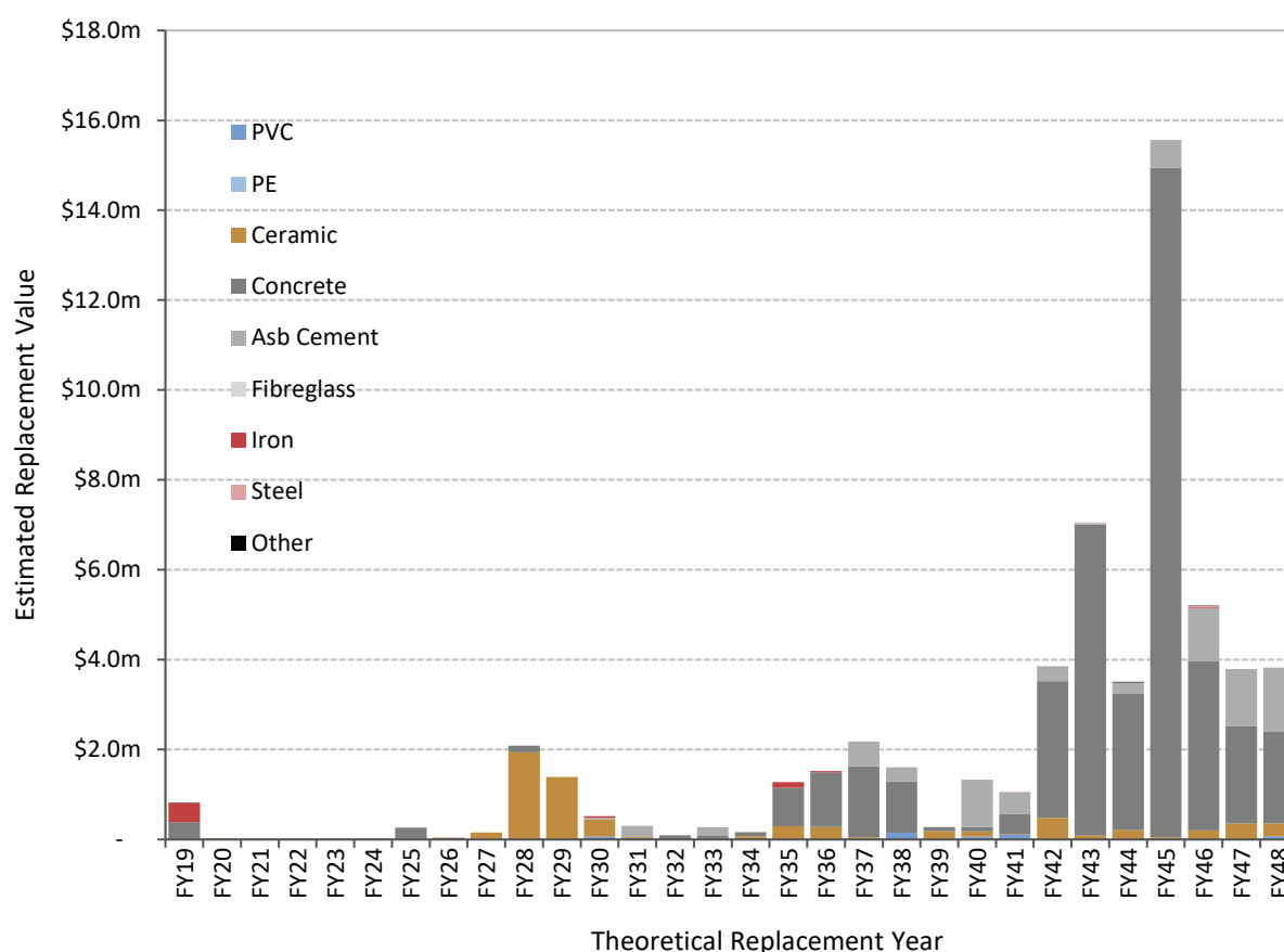
FIGURE 4: THEORETICAL WASTEWATER PIPE RENEWAL DATES
